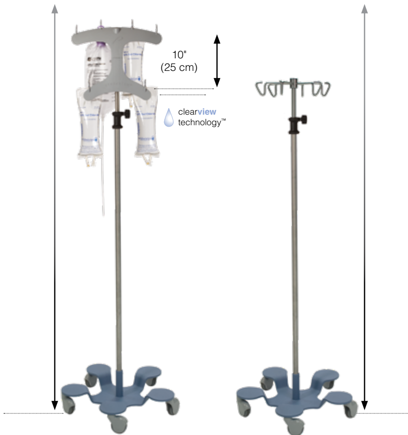
P-1080-CV Height adjustable from 71" to 124"
